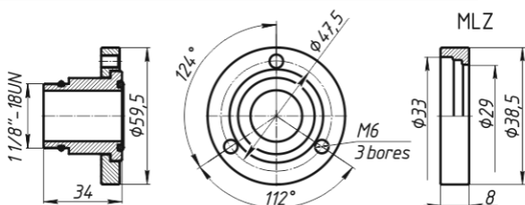
Adapter FP-ERL3/4-BBL(+MLZ).
