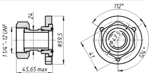
Adapter FP-ERL3/4-CEL.
