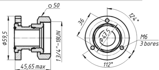
Adapter FP-ERL3/4-CD.
